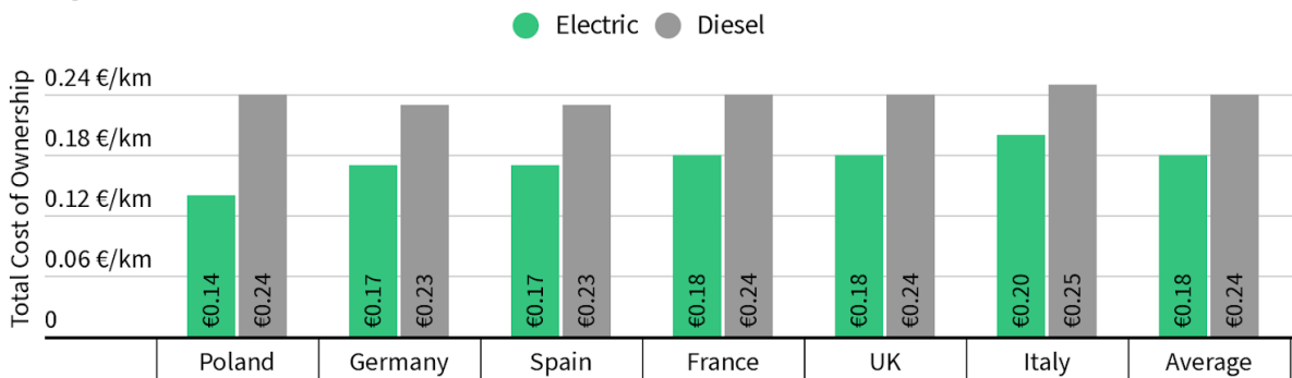
Figure 22: Average TCO of electric vans including subsidies and diesel vans in 2022 by country
